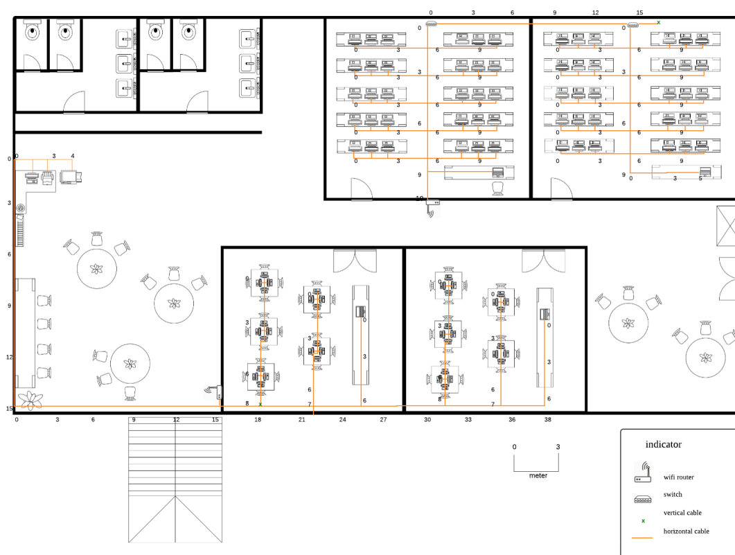
Figure 1: Ground floor plan with wiring
