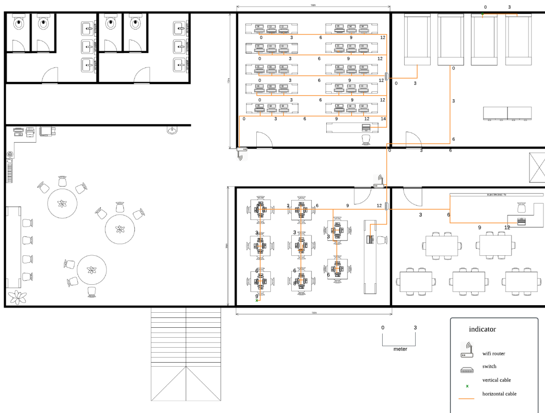
Figure 2: First floor plan with wiring
